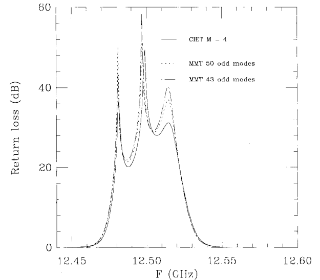
Fig. 4. Return loss (dB) of filter II as obtained from the CIET (solid line) with four basis functions and the MMT with 43 and 50 odd modes. The CIET reduces CPU time by a factor of 400.
